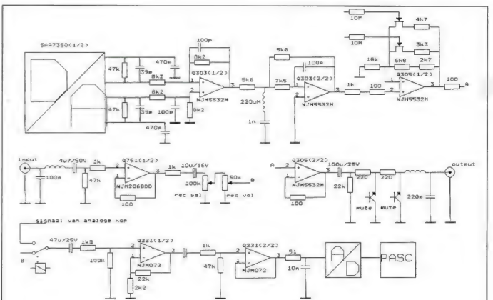
Technics RS-DC10
